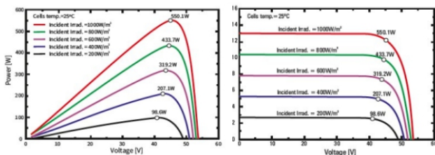
IV Curve Variation with irradiance
